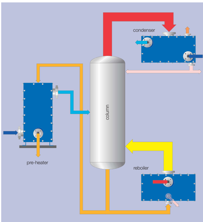
Compabloc as pre-heater, condenser and reboiler
