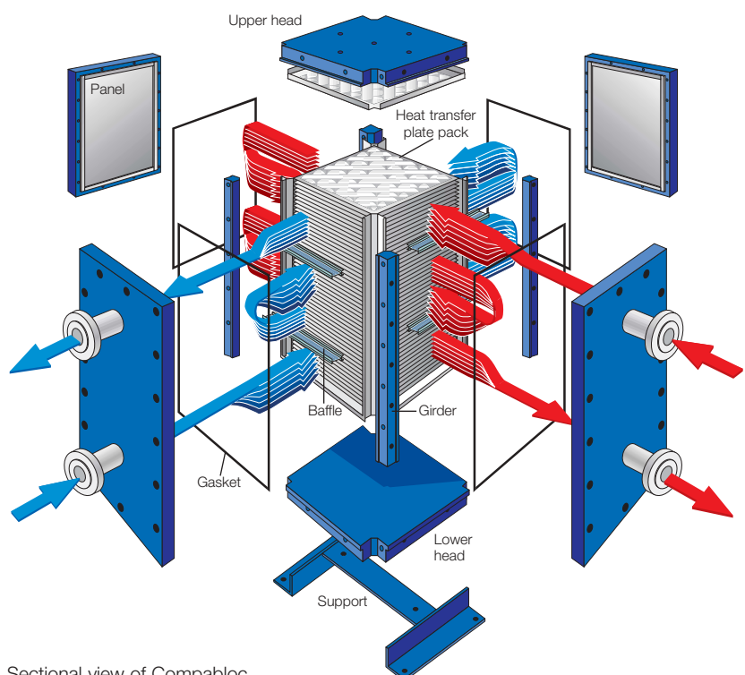
Sectional view of Compabloc
